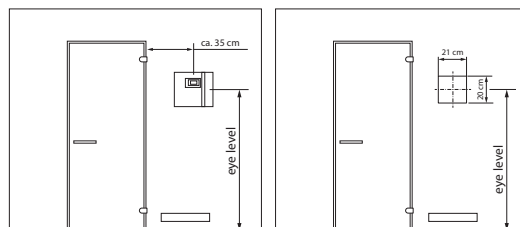
Wall cut-out (aperture) by semi-recessed mounting
